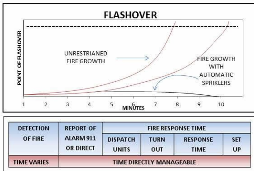
Figure 3: Typical Fire Flashover Timeline
